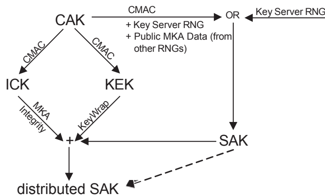
Figure 6-3—MKA key hierarchy
