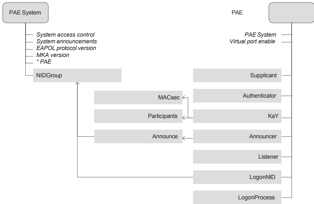
Figure 14-1—YANG model structure
