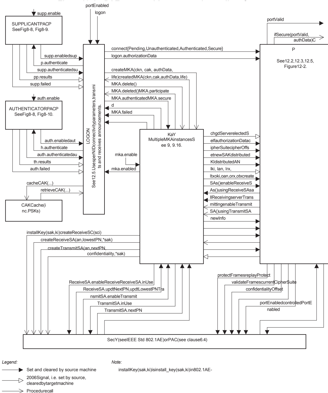
Figure 12-1—PAE state machines—overview and interfaces
