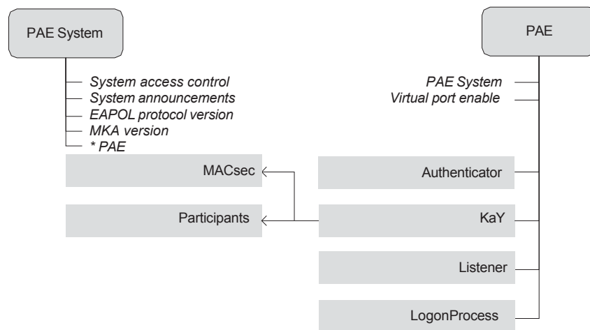
Figure 14-15—IEEE 802.1X YANG model for network access point (7.3)
