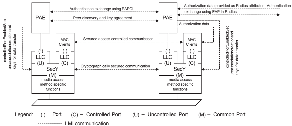
Figure 6-2—Port-based network access control with MACsec
