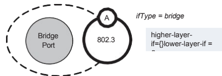
Figure 14-6—Augmented Interface Mode of Bridge Port.
