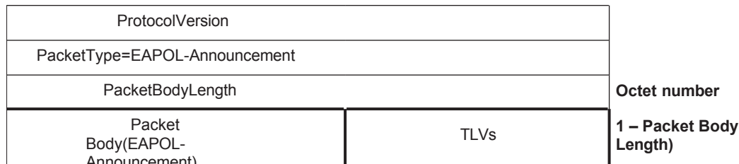
Figure 11-18—EAPOL-Announcement
